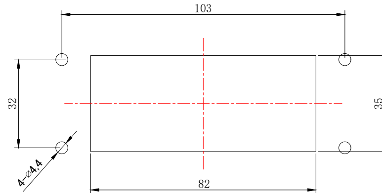
面板开孔图 Panel cut out
