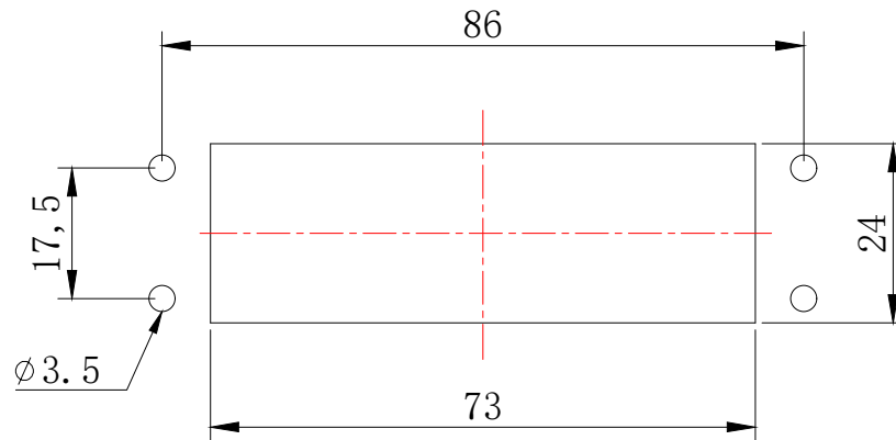
面板开孔图 Panel cut out
