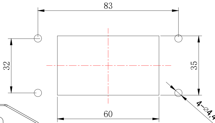
面板开孔图 Panel cut out
