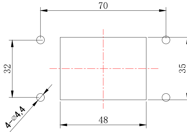
面板开孔图 Panel cut out
