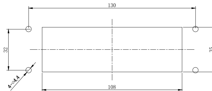
面板开孔图 Panel cut out
