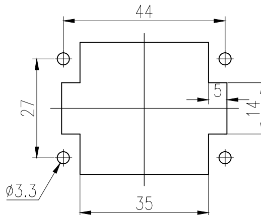
面板安装开孔图 Panel cut out
