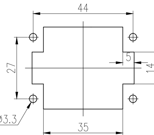
面板安装开孔图 Panel cut out
