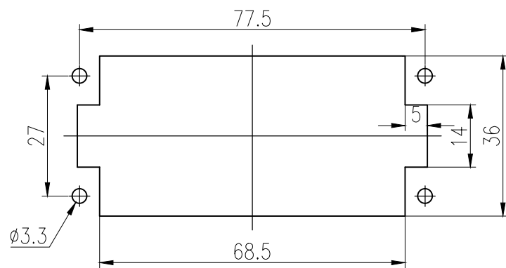
面板安装开孔图 Panel cut out
