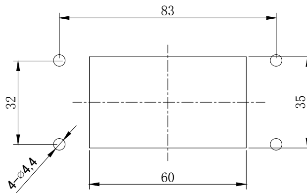
面板开孔图 Panel cut out
